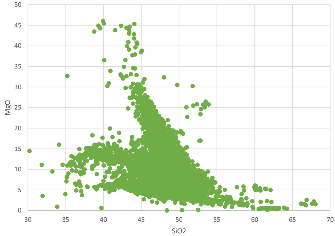
MgO vs. SiO 2
