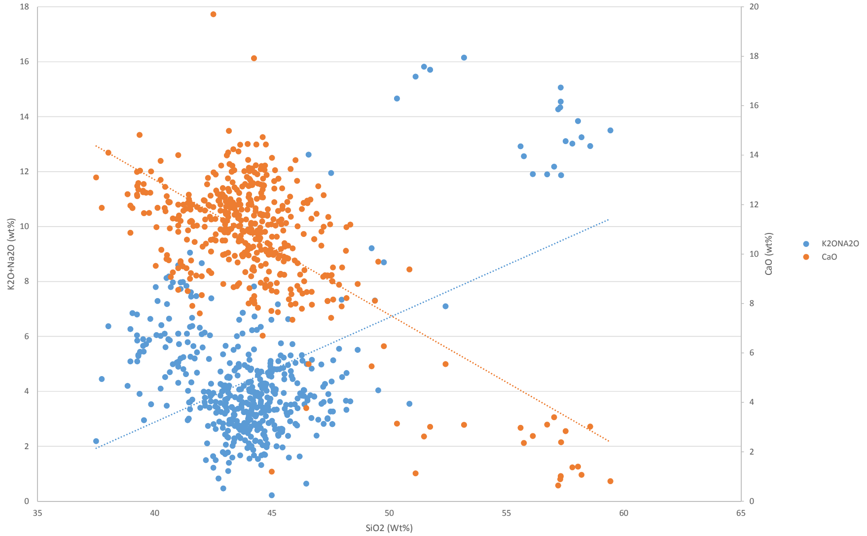
Total Alkalis and CaO vs. SiO 2
