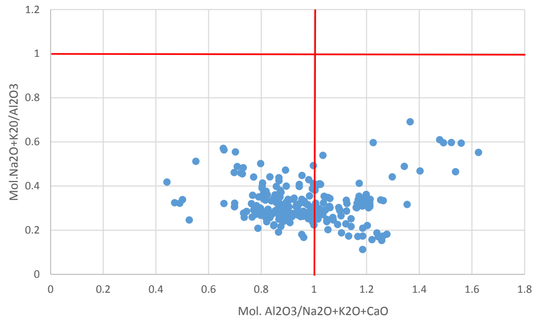
Alumina Saturation
