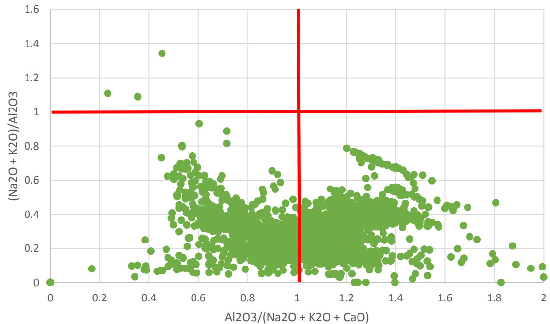
Aluminous Content
